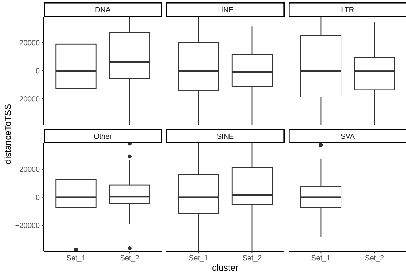
Distance to TSS by class in H3K27me3 of overlapping ROIs
